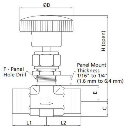
Straight Pattern
