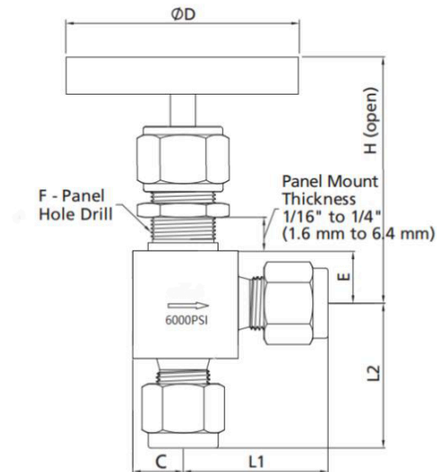
Angle Pattern
