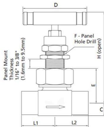
Straight Pattern
