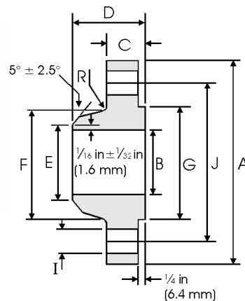
Weld Neck
