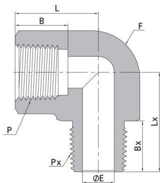
Female ISO Tapered Threads to Male ISO Tapered Thread
