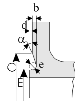
Type H 'O' Ring groove
