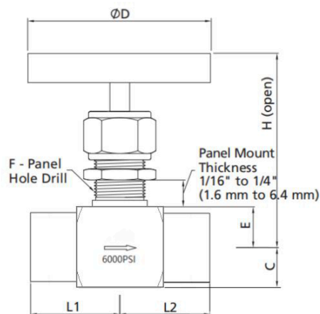
Straight Pattern
