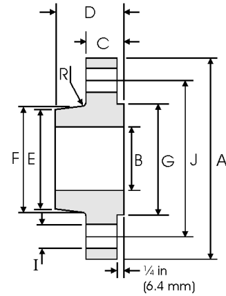
Slip On
