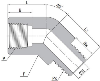
Female NPT Threads to Male NPT Thread
