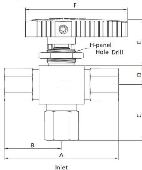
3-way
