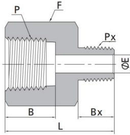
Female NPT Threads to Male ISO Tapered Threads
