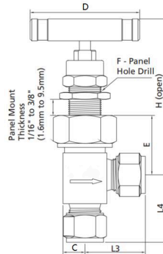
Angle Pattern
