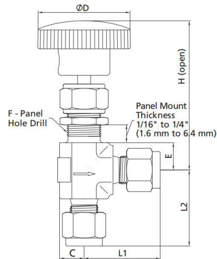
Angle Pattern
