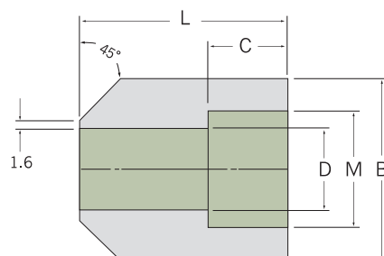
Boss
