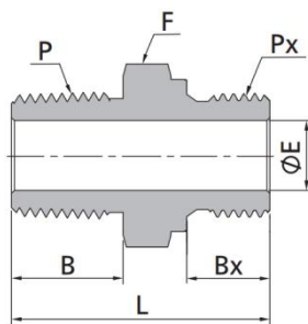
Male NPT Threads to Male ISO Parallel Threads
