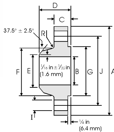
Weld Neck
