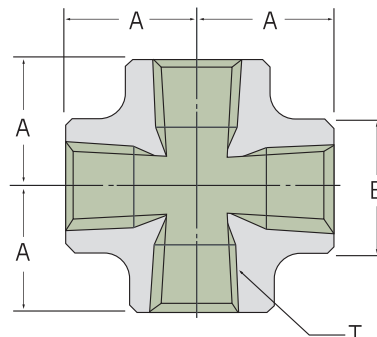
Cross
