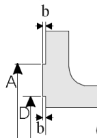
Type G 'O' Ring recess
