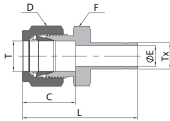
Metric Tube to Fractional Tube
