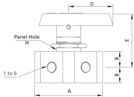
6-way Valve
