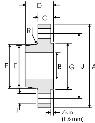
Slip On
