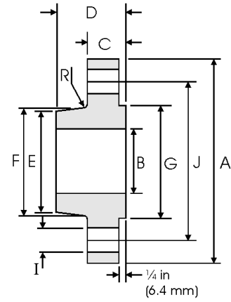
Slip On
