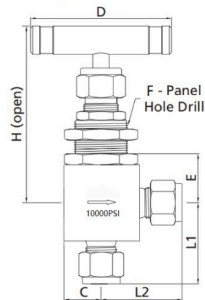
Angle Pattern
