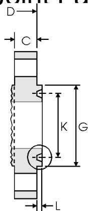
Ring joint facing dimensions - ASME/ANSI B16.5 and B16.47 Series A (MSS SP-44) and Series B (API 605) (Continued)
