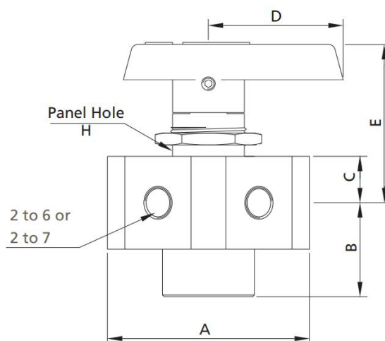
6, 7-way Valve
