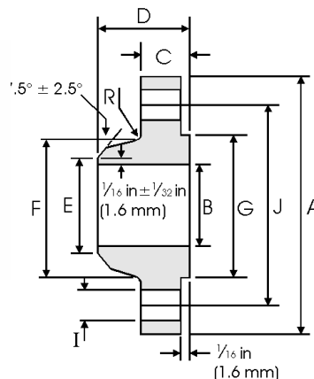
Weld Neck
