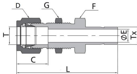
Fractional Tube
