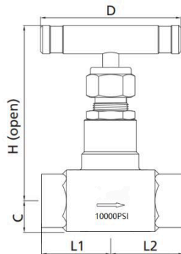
Straight Pattern
