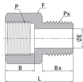
Female ISO Parallel Threads to Male NPT Threads
