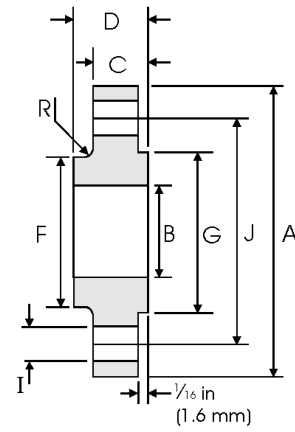
Slip On
