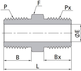
Male NPT Threads to Male ISO Tapered Threads
