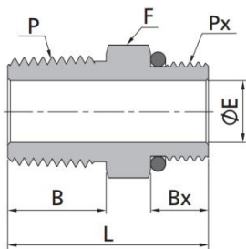
Male NPT Threads to Male ISO Parallel Threads
